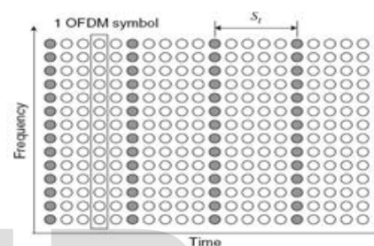
Figure .3(b) Block type Pilot
