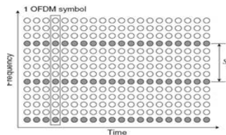
Figure .3(a) Comb Type Pilot
